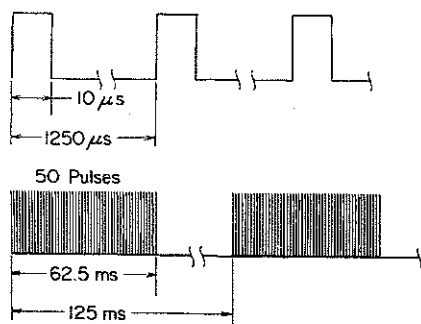
Fig. 3. Modulation characteristics of the microwave pulses: 8 groups per second, 50 10-μs-wide pulses per group, with a repetition rate of 800 pps. The period was 125 ms; with pulse onsets separated by 1.25-ms intervals. This is the equivalent of an 800-pps source square-wave modulated at 8 Hz.
