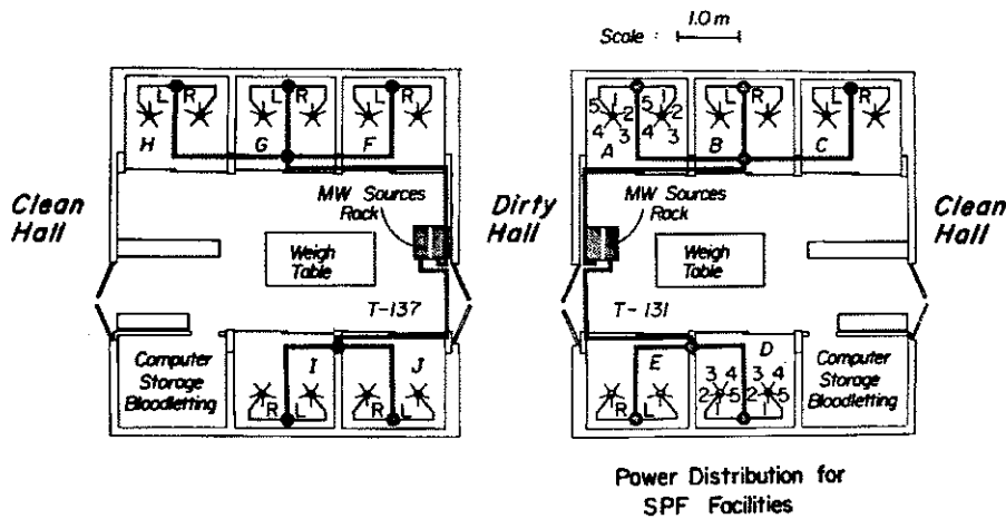
Fig. 1. Top view of exposure rooms (T-131 and T-137) with alcove designations and associated exposure-cell identification system.
